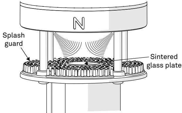
Figure 7 Anemometer
